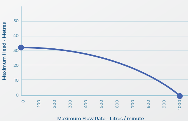
MH30-2 PUMP PERFORMANCE CURVE
