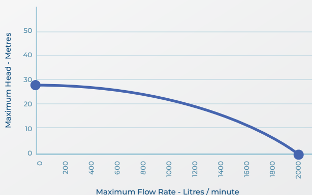
MH40TE-2 PUMP PERFORMANCE CURVE
