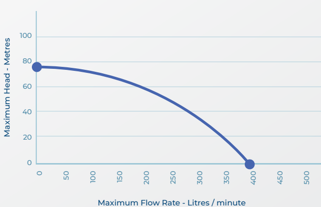
MHGP15-SHP PUMP PERFORMANCE CURVE
