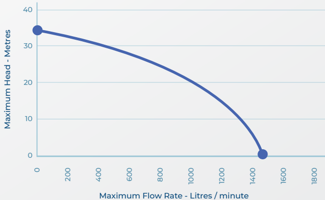
MH40-2 PUMP PERFORMANCE CURVE
